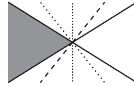
FIGURE 21 The generalized gradient is the set of all vectors enclosed by the adjacent surface gradients (solid lines). Three elements of the generalized gradient (dashed/dotted) in the nonsmooth point.
