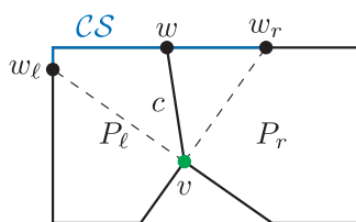
FIGURE 26 Cut space CS (blue) and decomposing cut c in the concave vertex v . Resulting in two polygons P_l and P_r , adapted from Bochkarev and Smith (2016).
