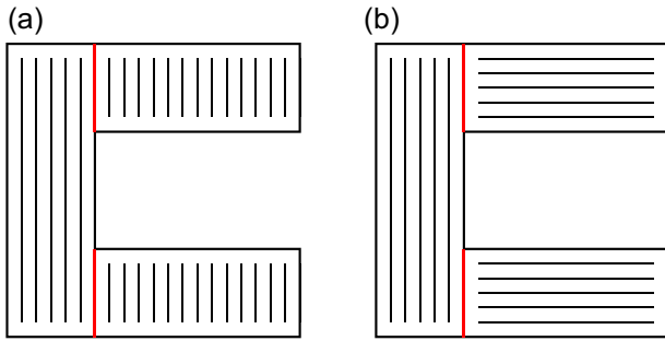
FIGURE 22 Decomposition of C-shaped region by vertical sweep line decomposition (red), and assigned track directions for each cell. (a) Track directions in all cells parallel to the sweep line and (b) track directions in each cell optimal w.r.t. the number of turns.
